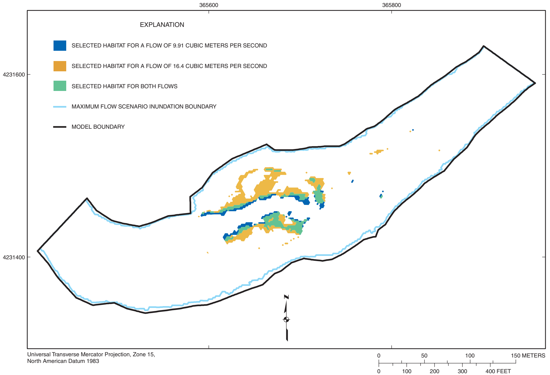
Figure 4-99. Selected habitat area distribution for habitat categories 24, 25 combined (stonecat) at flows of 9.91 and 16.4 cubic meters per second at Marais des Cygnes River site MDC2.
